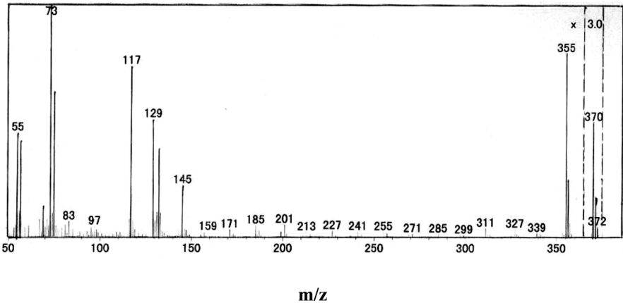
Fig. 3. Mass spectral profiles of nonadecanoic acid produced from n -eicosane by Trichoderma sp. S019.
