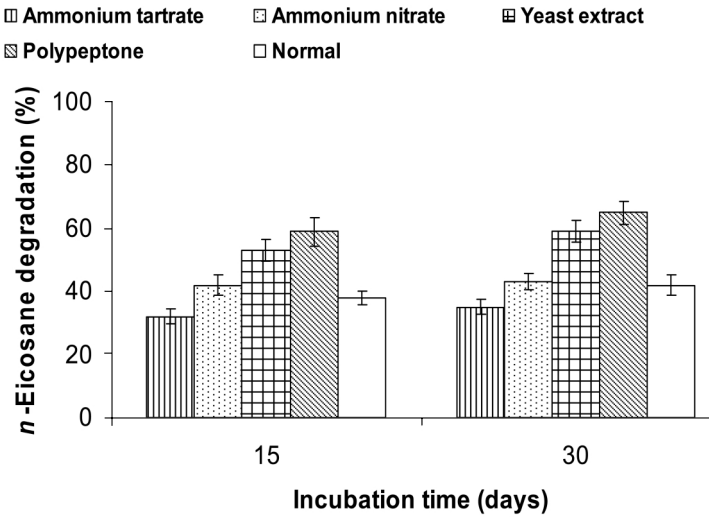
Fig. 2. Effect of nitrogen sources on degradation of n -eicosane in liquid medium by Trichoderma sp. S019.
