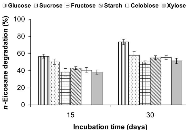
Fig. 1. Effect of carbon sources on degradation of n -eicosane in liquid medium by Trichoderma sp. S019.
