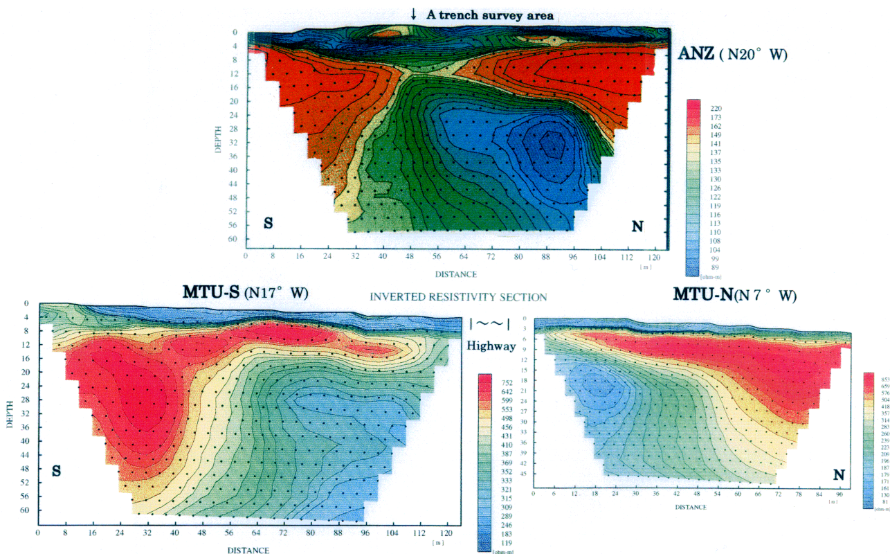
Fig. 3. (a) Resistivity cross-section of site ANZ (Top center). (b) Resistivity cross-section of site MTU-N (Right bottom). (c) Resistivity cross-section of site MTU-S (Left bottom). All figures are illustrated using a natural scale (V : E = 1 : 1). Dots show data points.
