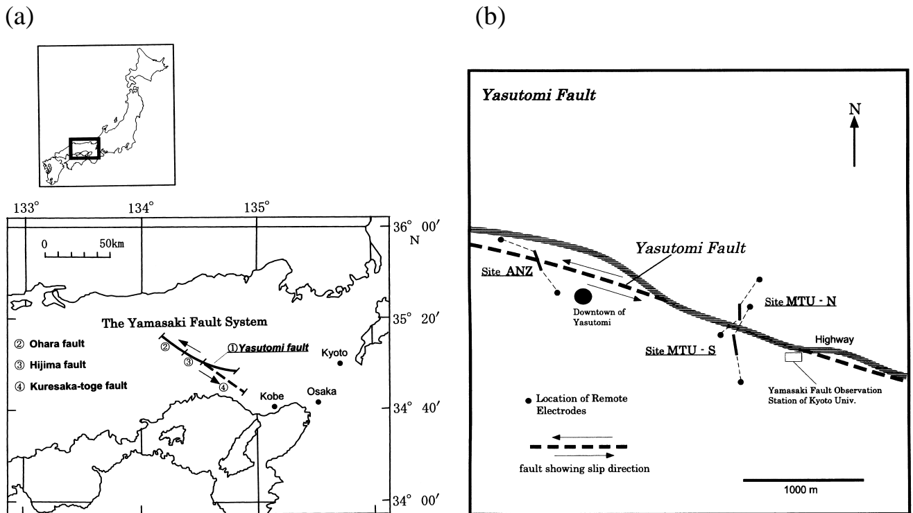
Fig. 1. (a) Location map showing the Yamasaki fault system. Yasutomi fault is situated in the middle of the Yamasaki fault system. (b) Configurations of Multi-Electrodes Resistivity profiles. An Anzi (ANZ) profile is designed to cross the Yasutomi fault. Mitsumori-North (MTU-N) and Mitsumori-South (MTU-S) profiles are separated to avoid the effect of the highway and its base.
