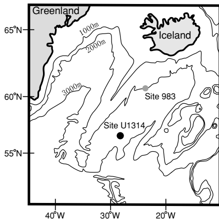
Fig. 1. Location map for IODP Site U1314, which is about 500 km from ODP Site 983 downstream the Gardar Drift. Bathymetric contours are given in meters.
