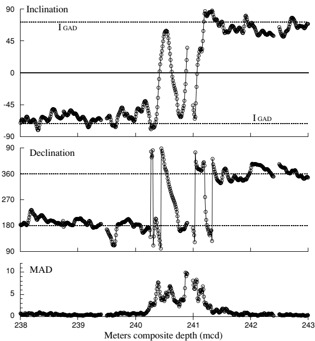
Fig. 4. Principal components (declination and inclination) and maximum angular dispersion (MAD). Inclination expected from geocentric axial dipole at the sampling site is indicated as I_{GAD} .
