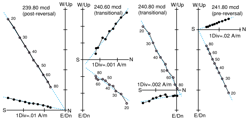
Fig. 3. Examples of orthogonal projections of alternating field demagnetization. Solid circles represent the horizontal projection, and open circles represent the vertical projection. The peak alternating field (mT) for each demagnetization step is indicated. Dotted lines indicate calculated component directions.
