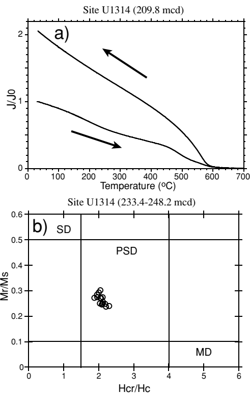
Fig. 2. (a) Typical result of thermomagnetic analysis. (b) Hysteresis ratio plot for 15 samples. SD, PSD, and MD indicate single domain, pseudo-single domain, and multidomain fields, respectively (see Day et al. , 1977).
