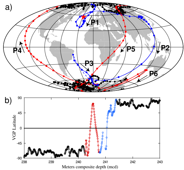
Fig. 5. Virtual geomagnetic poles (VGPs) during the G-M transition. (a) Path plotted on Hammer projection. The arrows indicate the movement of VGPs, and P1 to P6 represent the temporal order. Star indicates the drilling site. (b) VGP latitudes as a function of depth.
